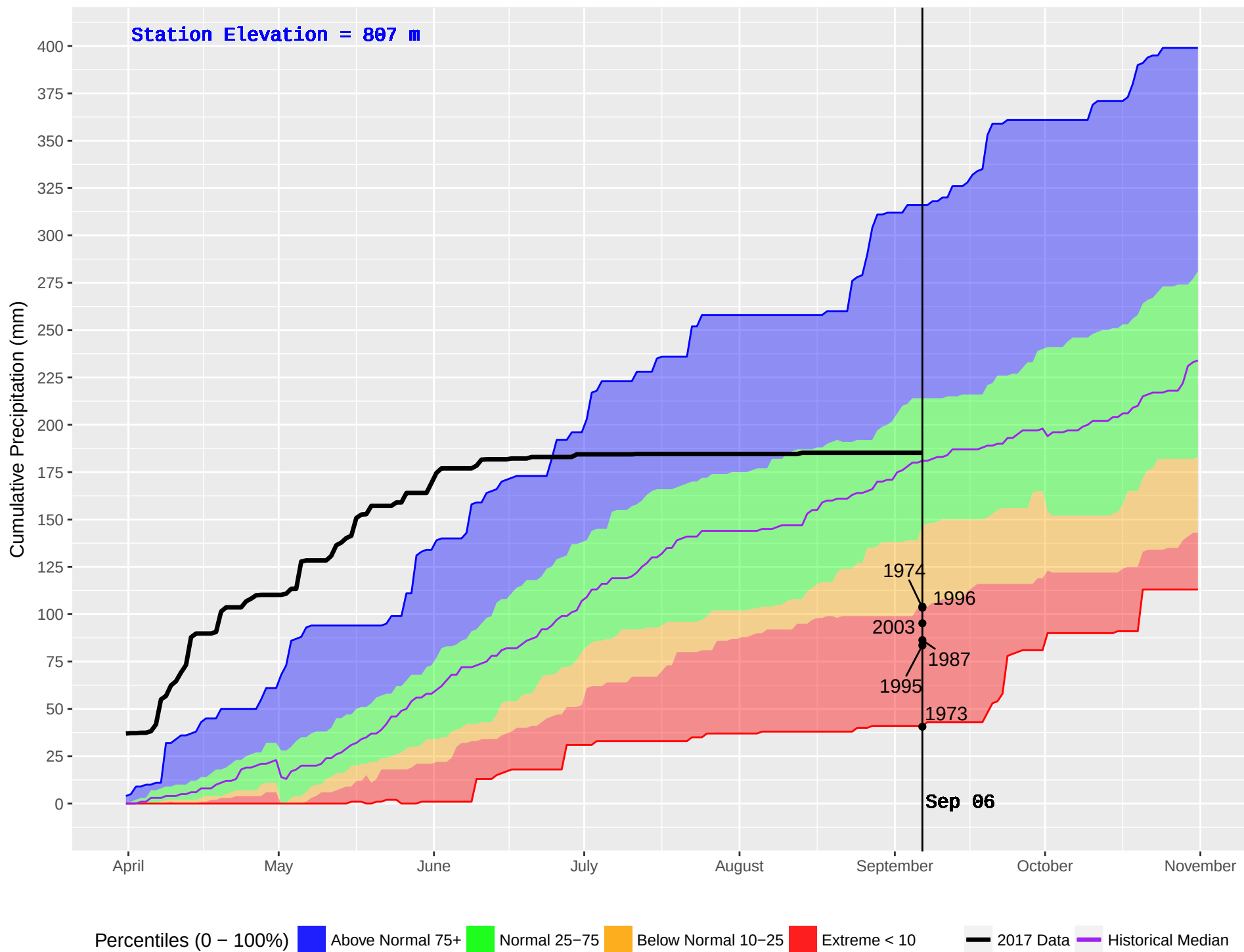
BEAVERDELL (390) : Historical (1970–2016) and Current (2017) Noon Cumulative Precipitation
