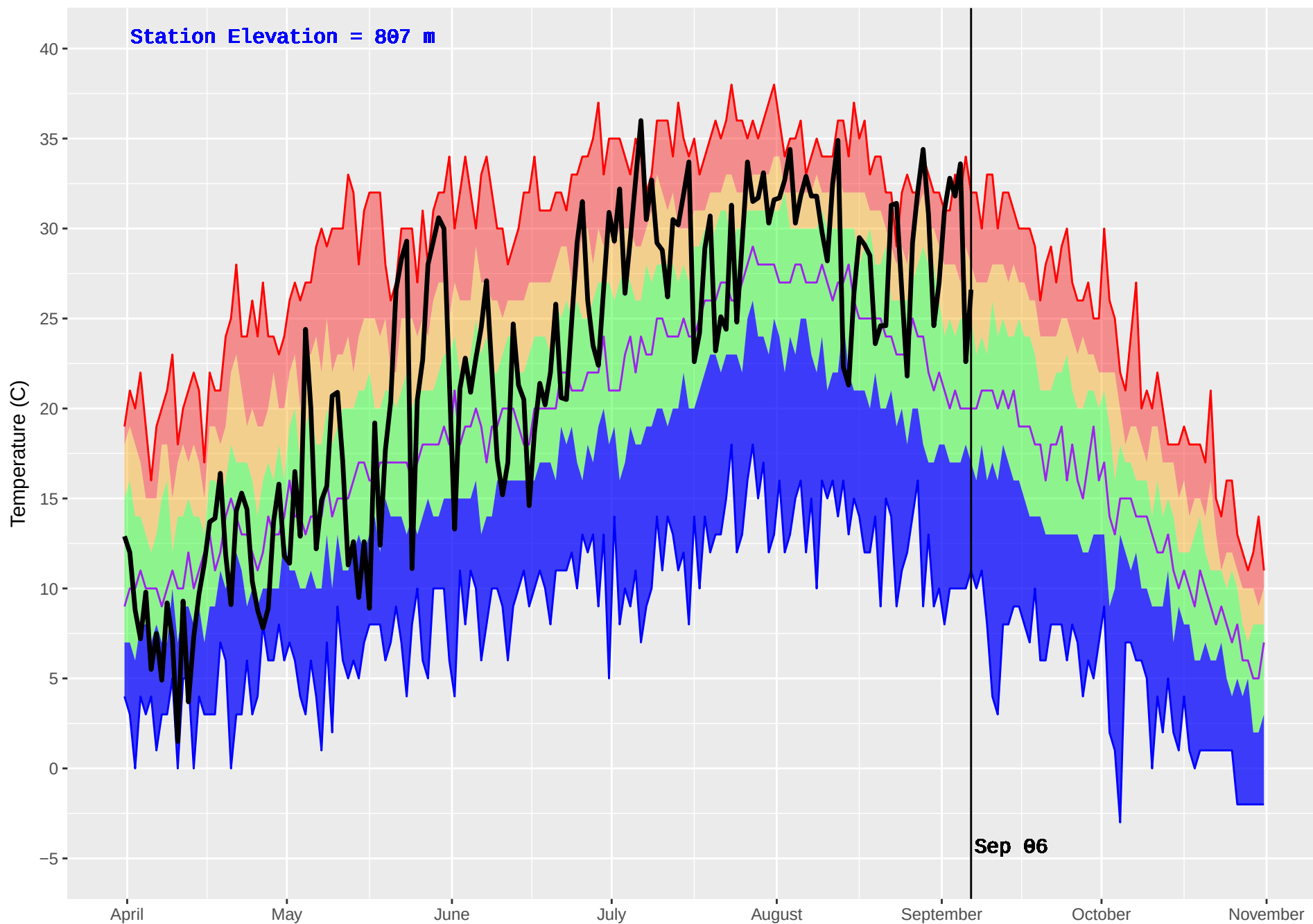
BEAVERDELL (390) : Historical (1970–2016) and Current (2017) Noon Temperature
