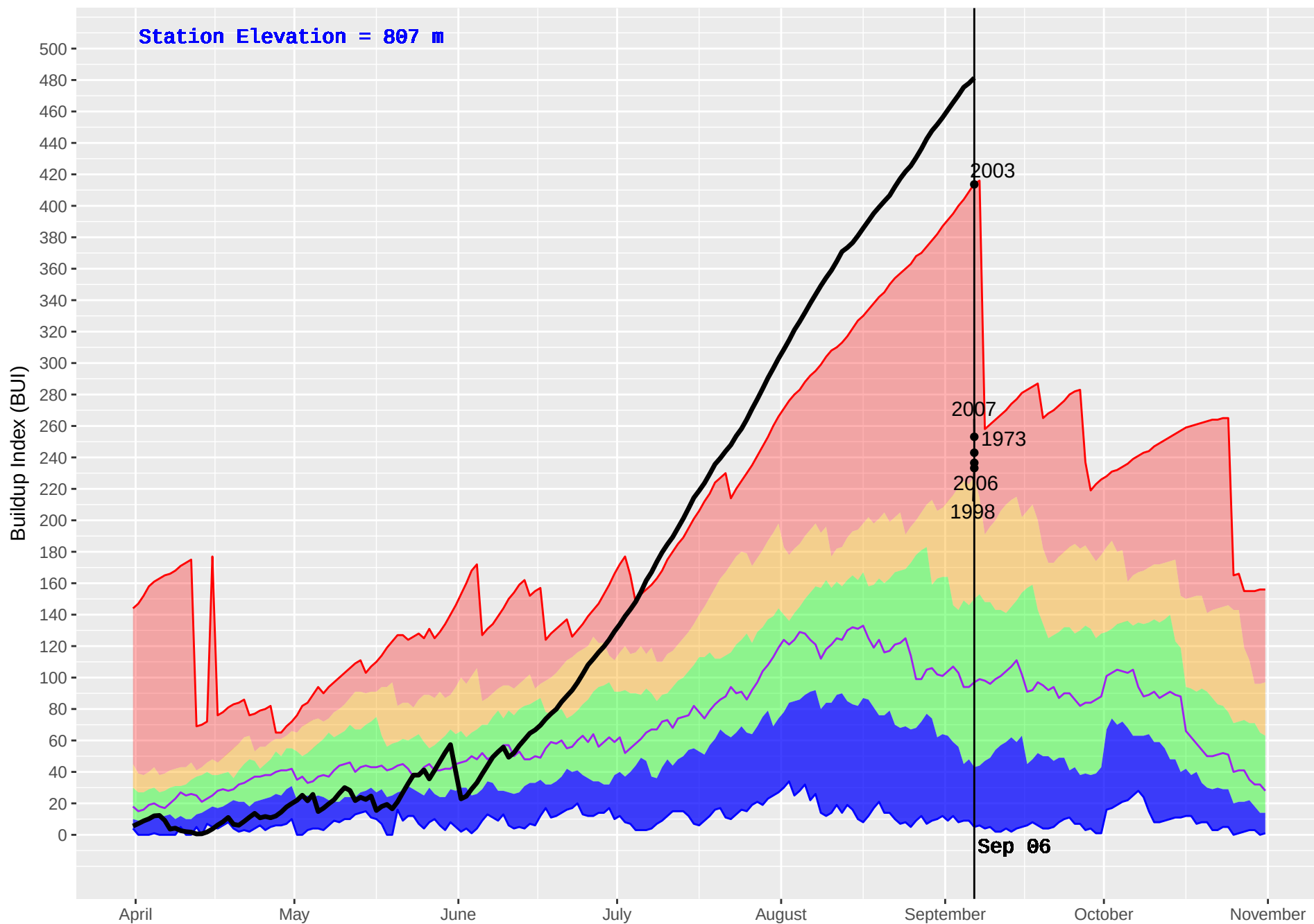
BEAVERDELL (390) : Historical (1970–2016) and Current (2017) Noon Buildup Index (BUI)
